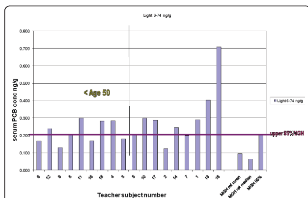
Figure 1 Serum concentrations of light congeners (PCB 6-74), teachers compared to MGH referent values.
