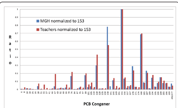
Figure 2 Comparison of median serum congener concentrations normalized to congener 153 concentration between teachers and MGH referents. Comparison of the height of the two bars (teachers and referents) for each congener illustrates the differences in the relative abundance of each congener in the serum of the teachers and the referents. The greatest differences are apparent in the lighter congeners, PCB 6-74, where the teachers' values consistently exceed the referents.
